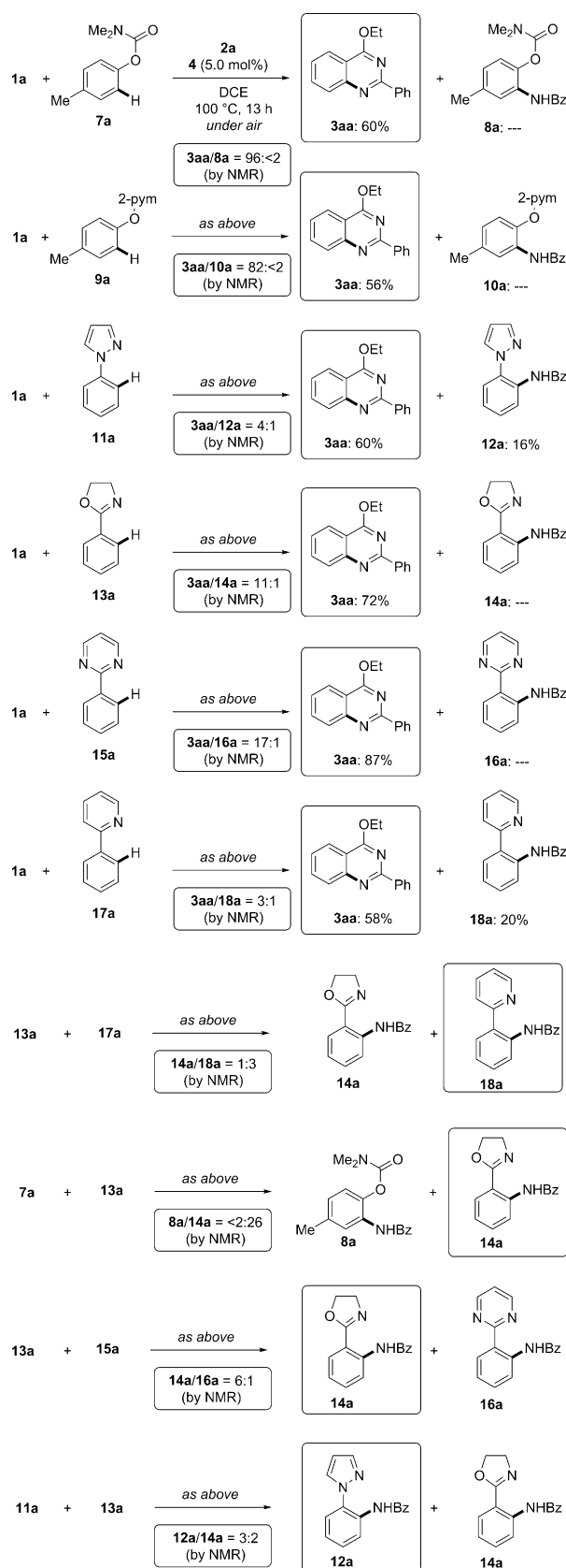
Scheme 3. Directing group powers in cobalt-catalyzed C–H functionalization; yields of isolated products are given. Product ratios were determined by 1 H NMR spectroscopy with 1,3,5-trimethoxybenzene as the internal standard. Bz = benzoyl, 2-pym = 2-pyrimidyl.
