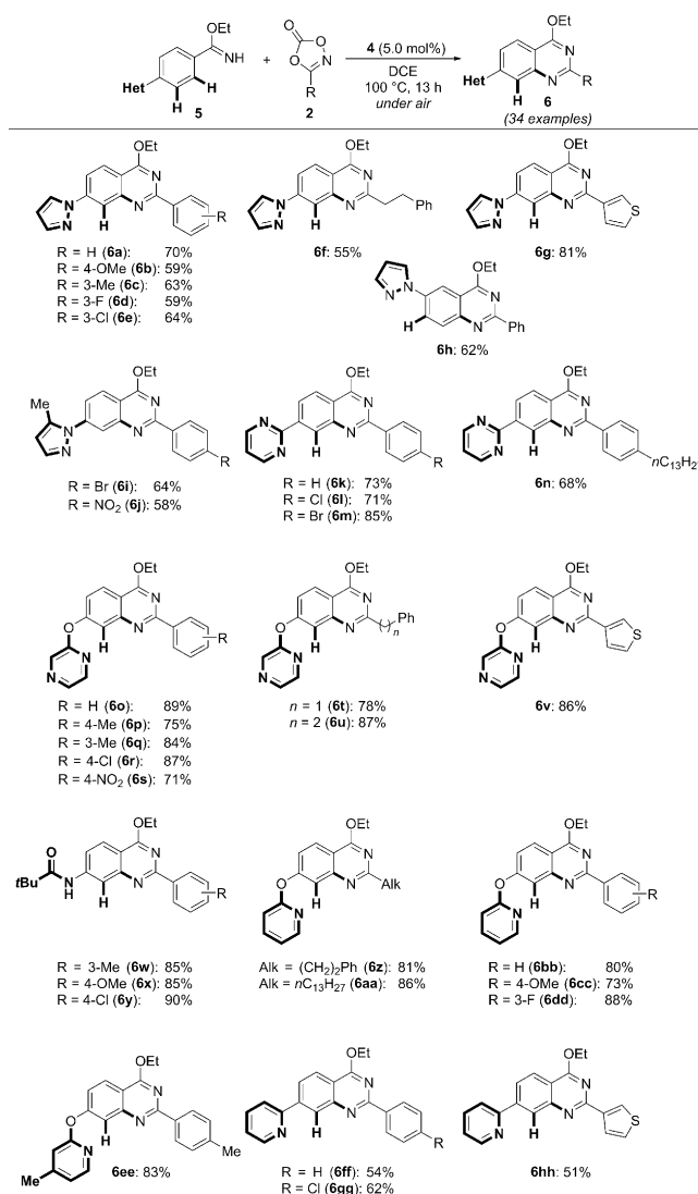
Scheme 2. Overriding the conventional selectivity dictated by strongly coordinating heterocycles.
