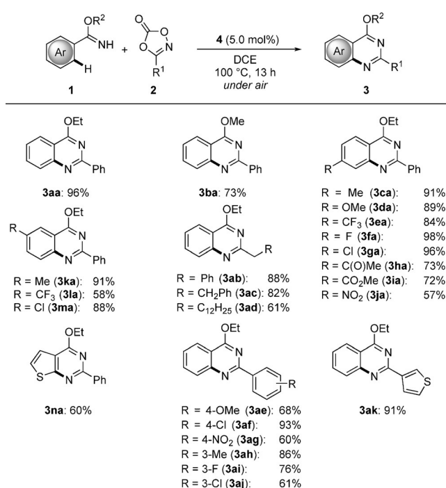
Scheme 1. Cobalt-catalyzed C–H nitrogenation of imidates 1 .
