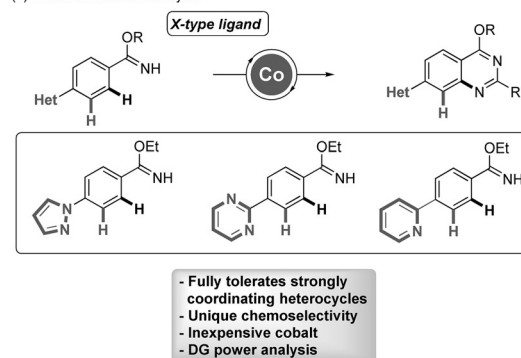
Figure 1. C–H activation in the presence of strongly coordinating heterocycles. a) Challenges. b) Palladium(II) catalysis. [5] c) Heterocycle-tolerating cobalt catalysis.
