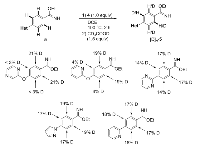
Scheme 4. Positional selectivity in stoichiometric C–H cobaltation.
